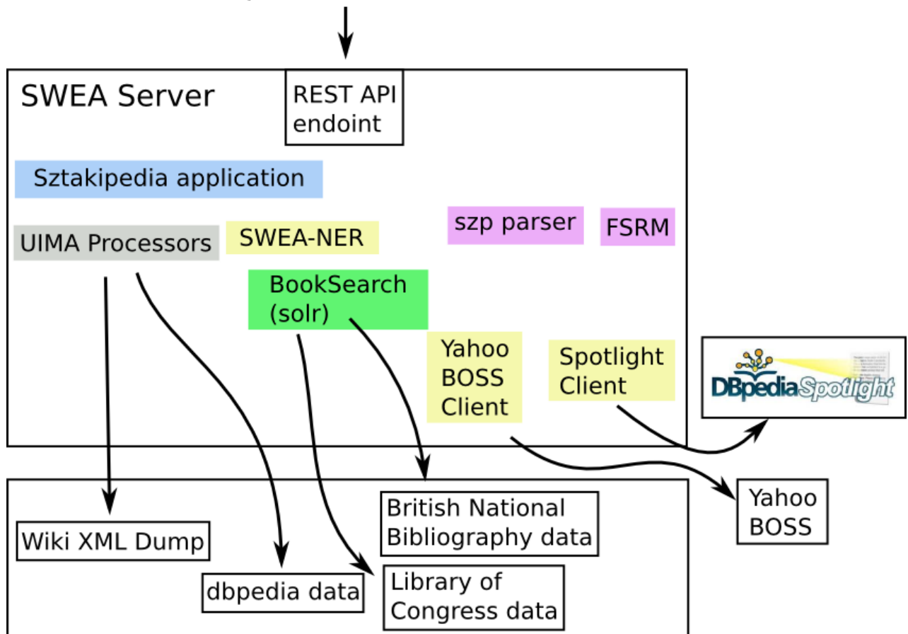
Figure 2: The Architecture of Sztakipedia
