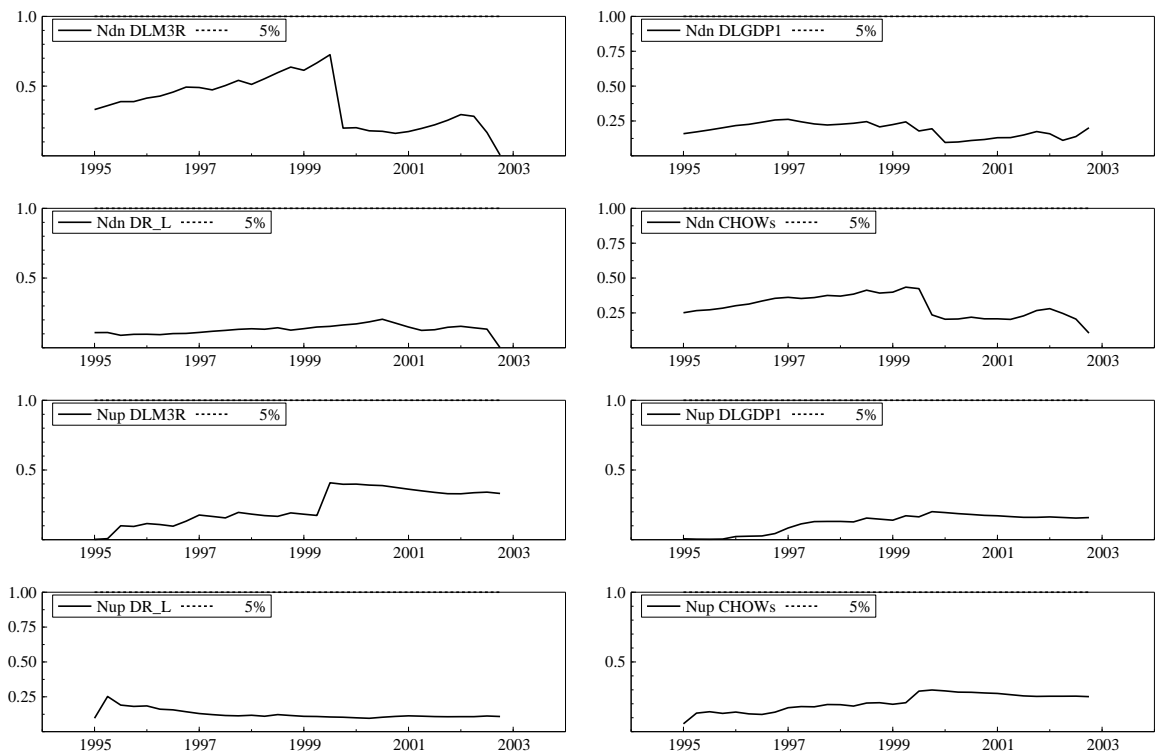
Figure A.2: Results from single equation and system breakpoint ( Ndn ) and forecast ( Nup ) Chow-tests for VECM with 2 lagged differences. Sample period 1984Q1-2002Q2. Computations performed with PcGive 10.3 (see Doornik & Hendry (2001) for details).
