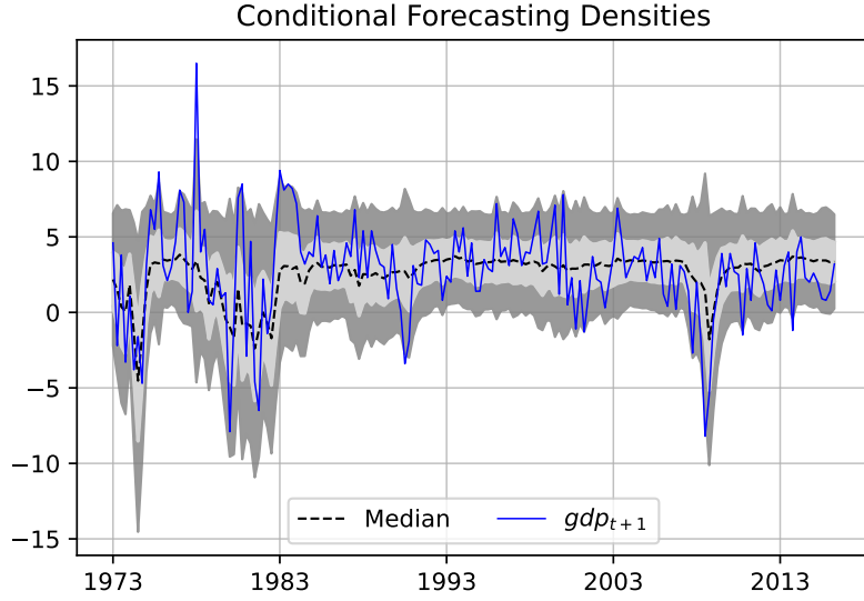
Figure 6: The one-step ahead forecasting distribution for one-quarter ahead GDP growth Notes: Lower and upper 5% and 25% percent quantiles display the same characteristics as found by Adrian et al. (2019). While the upper quantiles remain relatively stable, the lower quantiles vary strongly over time indicating increased downside risks to GDP growth in times of financial distress.
