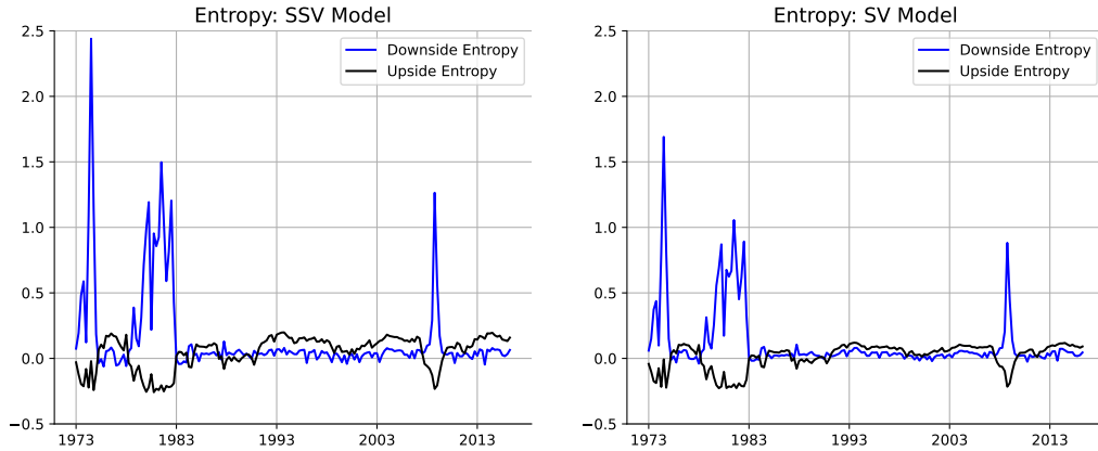
Figure 8: Filtered states obtained with the tempered particle filter
