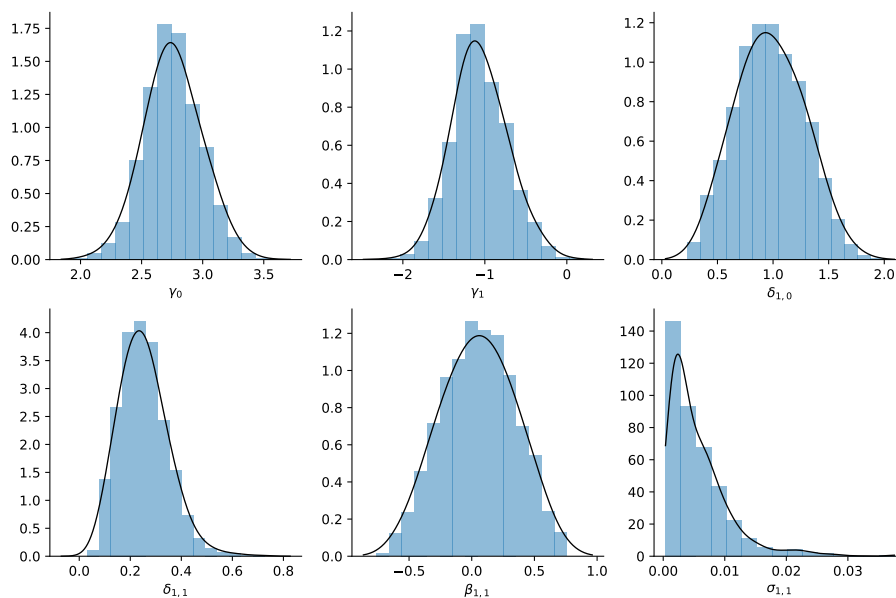
Figure 12: Stochastic Volatility Models: Posterior Distributions
