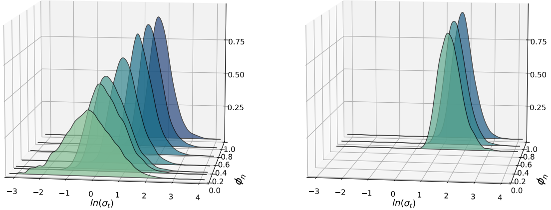
Figure 2: Tempering of the state distributions of \ln(\sigma_{t,i}^2) in 1978 (Q2)
