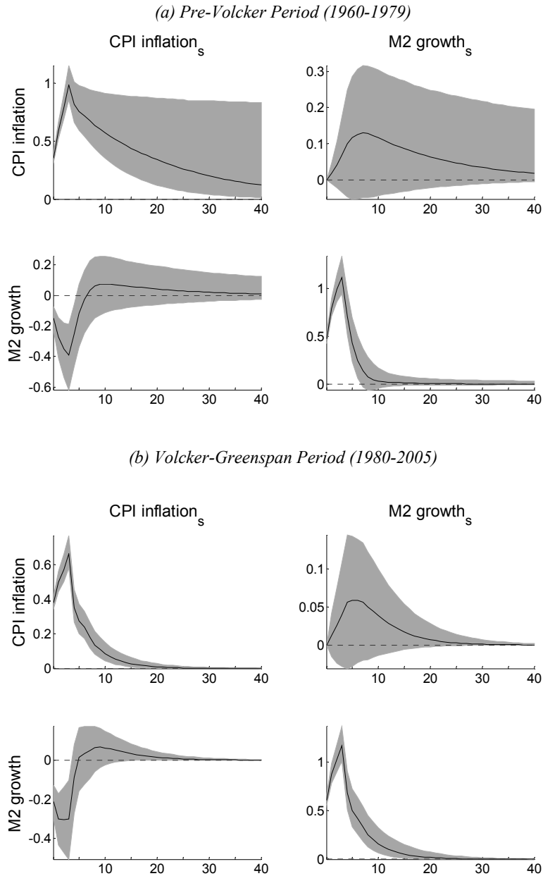
Figure A1. Impulse response functions from bivariate BVAR models including money growth and inflation, 1960-1979 and 1980-2005.
